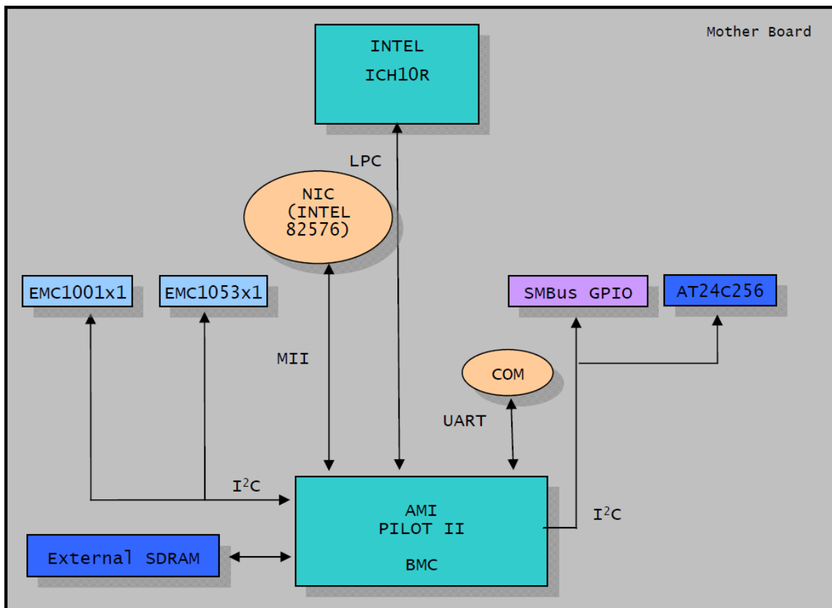
Figure 29. System Block Diagram
