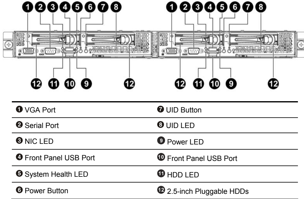
Figure 3. System Front View
