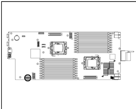
Figure 21. Location of MISC Jumper
