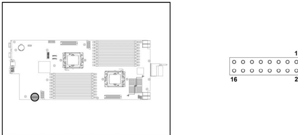
Figure 23. MISC Jumper
