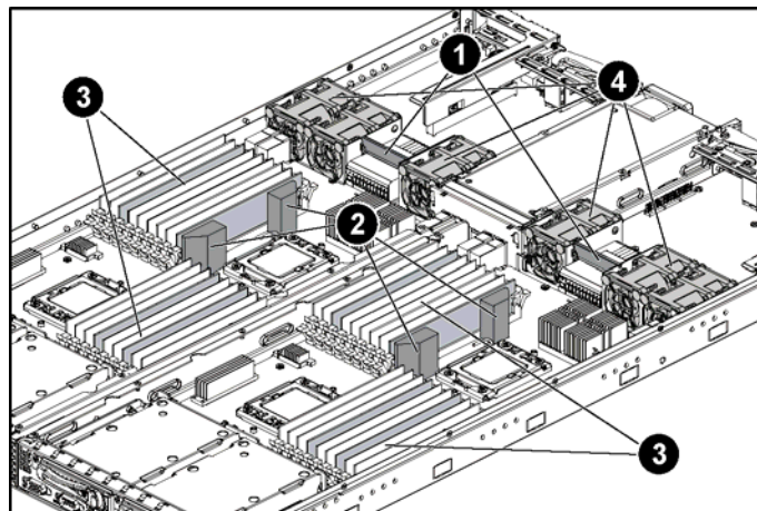
Figure 13. System Fans and Air Ducts
